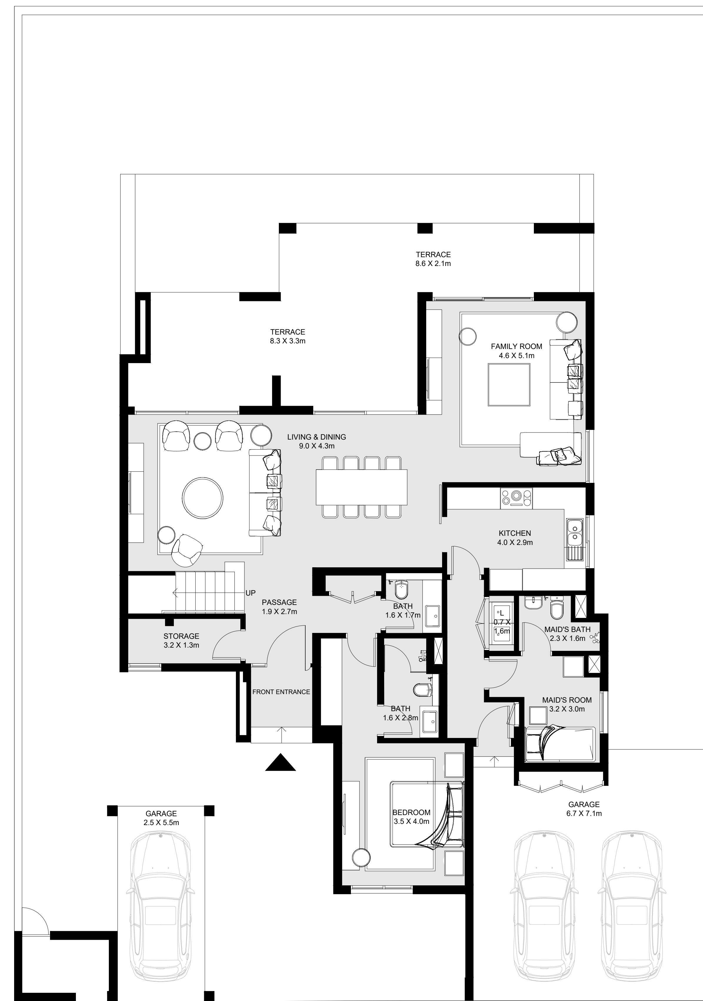
GROUND FLOOR
